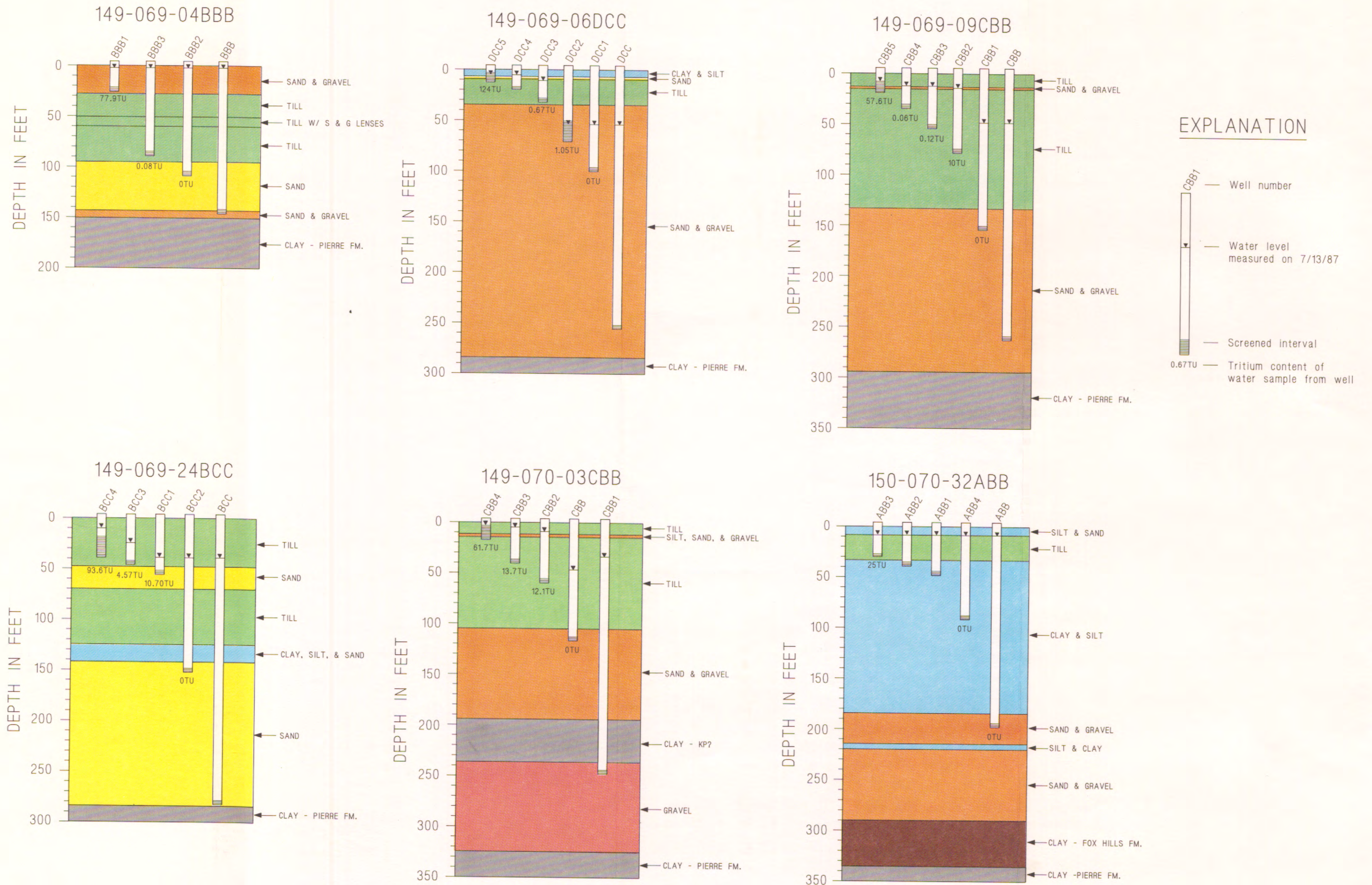
FIGURE 11. Nest site sections showing lithologies and tritium values. (hydrogeology by J.C. Patch)
