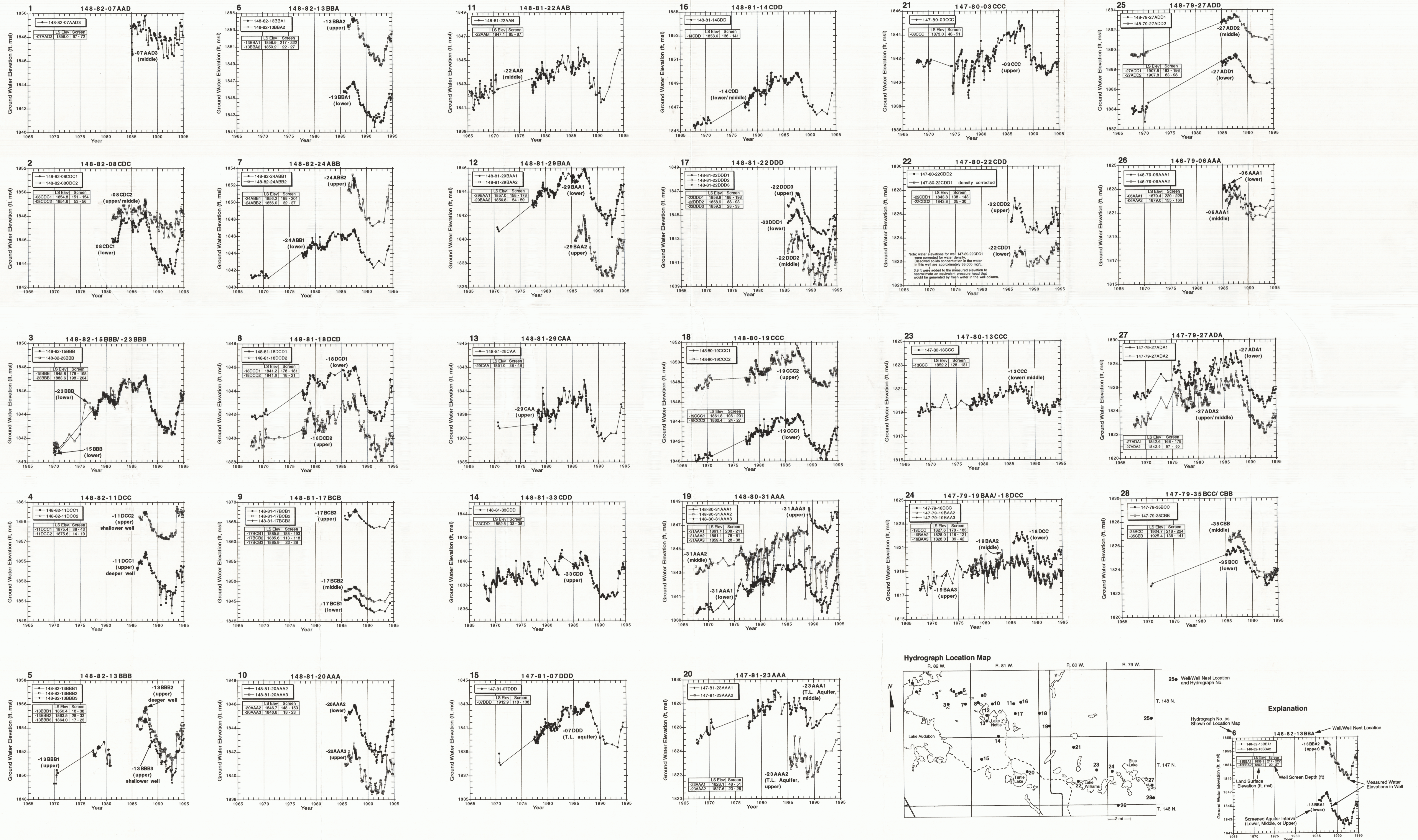
Plate 2. Representative Hydrographs Showing Water Level Elevations in Observation Wells in the Lake Nettie and Turtle Lake Aquifers
